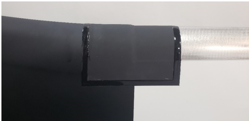
Figure 4 ~ Completed Polyurethane Tape Installation – Inboard Abrasion Strip Joint
